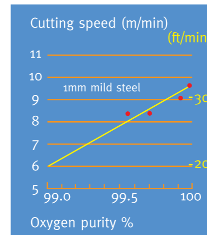
FIGURE 9: Effect of oxygen purity on the cutting speed for 1mm (0.04 in) mild steel using 800 W laser power and cutting oxygen pressure of 3 bar (44 psi)
