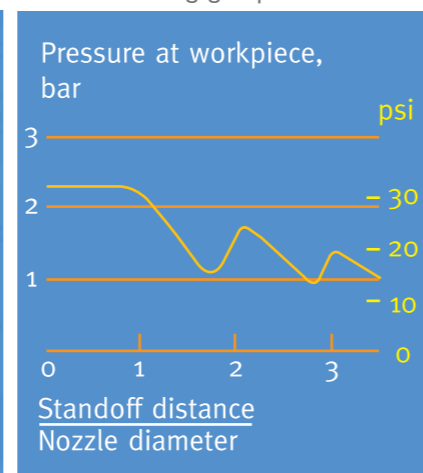
FIGURE 8: Effect of nozzle parameters on effective cutting gas pressure
