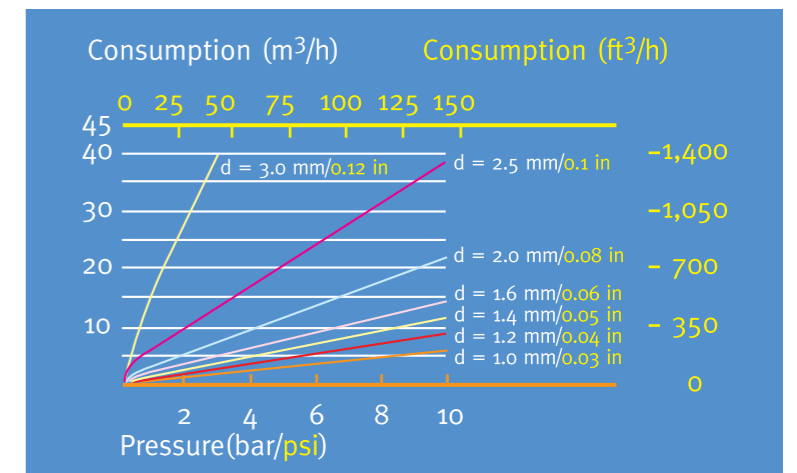
FIGURE 10: Consumption of oxygen depending on the gas pressure in the nozzle and the size of the nozzle, d
