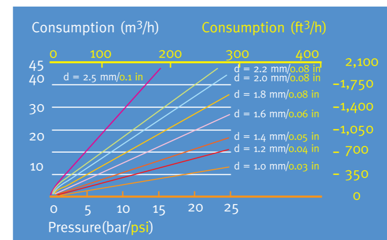
FIGURE 12: Consumption of nitrogen depends on the gas pressure in the nozzle and the size of the nozzle, d
