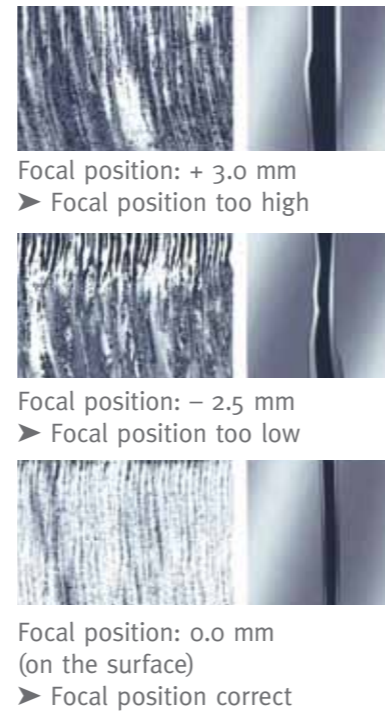
FIGURE 6: An illustration of the effect of focal position on cutting performance
