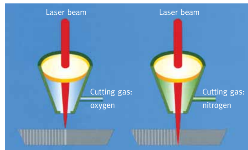
FIGURE 11: Focus position for oxygen-cutting compared to high-pressure nitrogen-cutting
