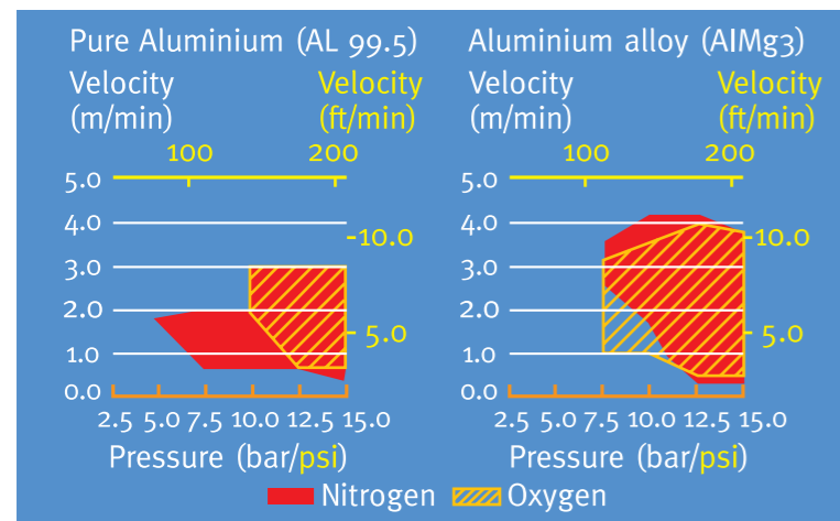
FIGURE 13: Dross-free parameter ranges when using nitrogen and oxygen up to 15 bar (217.5 psi) for cutting 2 mm (0.08 in) pure aluminium and 2 mm (0.08 in) aluminium alloy, laser power 1500 W
