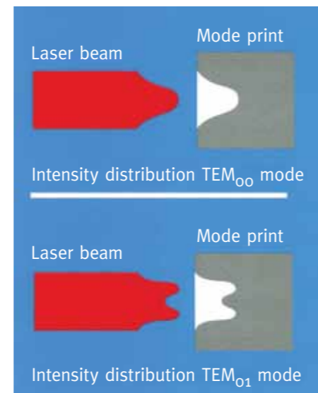
FIGURE 4: Intensity distribution across the laser beam
