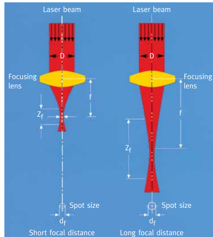
FIGURE 3: Focusing a laser beam
