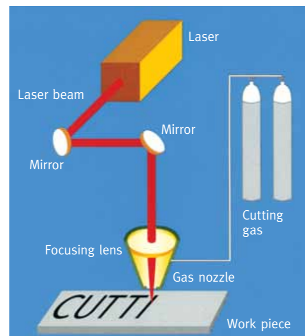
FIGURE 1: Principles of a laser cutting system (schematic)
