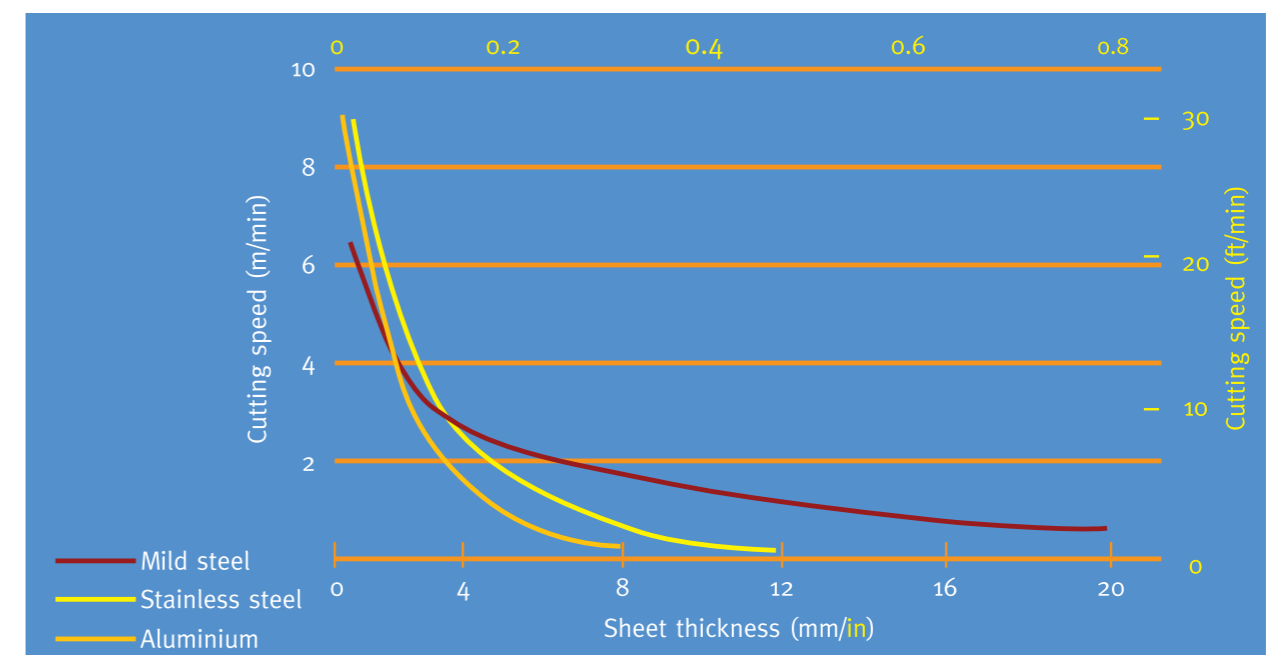
FIGURE 2: Typical cutting rates with approximately 3 kW of laser power
